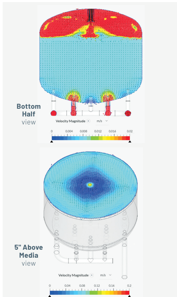
Yardney GAC 144 inch
