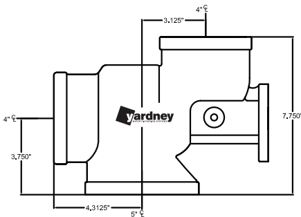
454 VALVE USED ON 36", 48" & 54" TANKS
