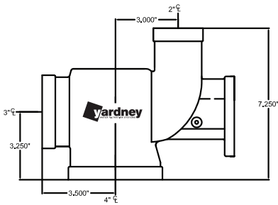
342 VALVE USED ON 24" & 30" TANKS
