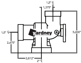
1-1/2" VALVE USED ON 14" & 18" TANKS
