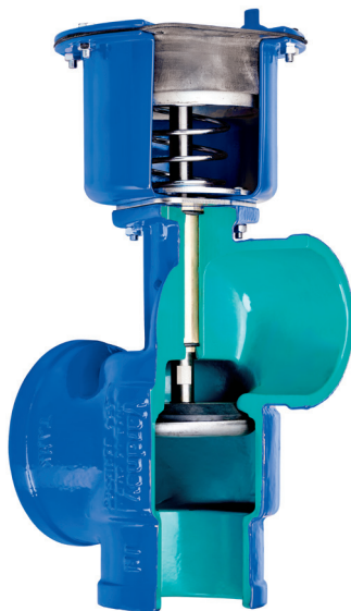
(cutaway view)
