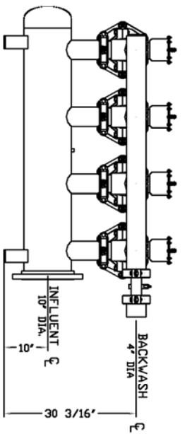
LEFT END VIEW
